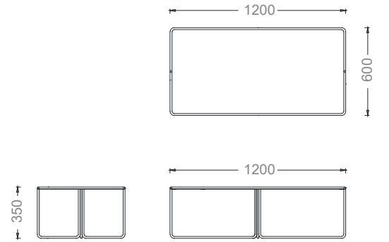
PLT12060- PLANET DİKDÖRTGEN SEHPA 120x60x35h
