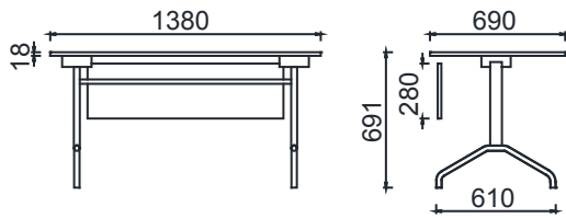
FD70140- FOLD FOLDING TABLE 70x140
