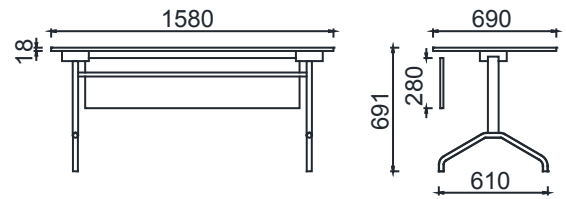
FD70160- FOLD FOLDING TABLE 70x160
