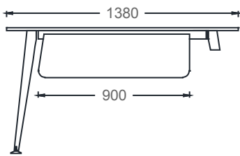
M3O70140 - MIO THREE-LEGGED SINGLE DESK 70x140
