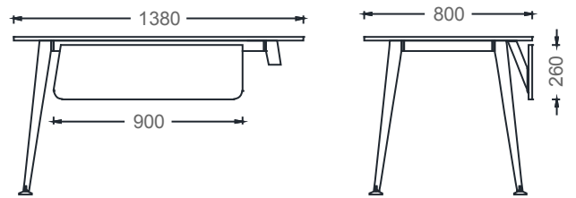
MEO80140 - MIO SIDE-UNIT DESK 80x140
