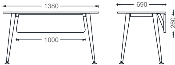
M4070140 - MIO SINGLE DESK 70x140
