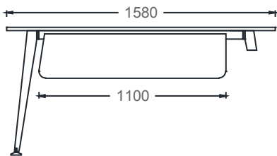
M3O70160 - MIO THREE-LEGGED SINGLE DESK 70x160
