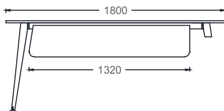
M3O80180 - MIO THREE-LEGGED SINGLE DESK 80x180
