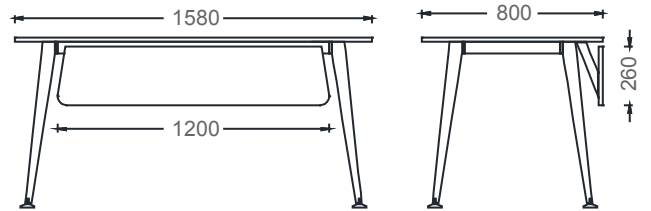
M4080160 - MIO SINGLE DESK 80x160
