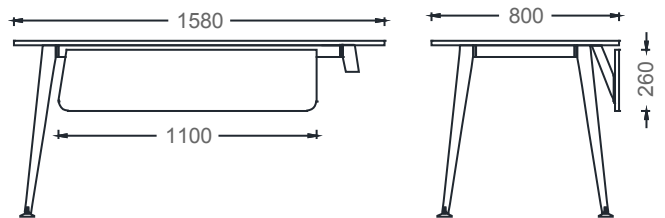
MEO80160 - MIO SIDE-UNIT DESK 80x160
