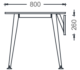
M3O80140 - MIO THREE-LEGGED SINGLE DESK 80x140
