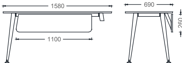
MEO70160 - MIO SIDE-UNIT DESK 70x160
