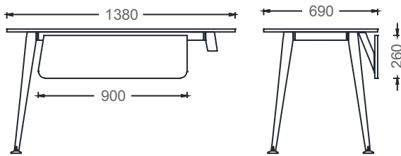
MEO70140 - MIO SIDE-UNIT DESK 70x140
