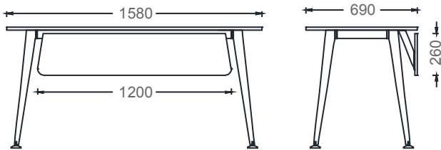
M4070160 - MIO SINGLE DESK 70x160
