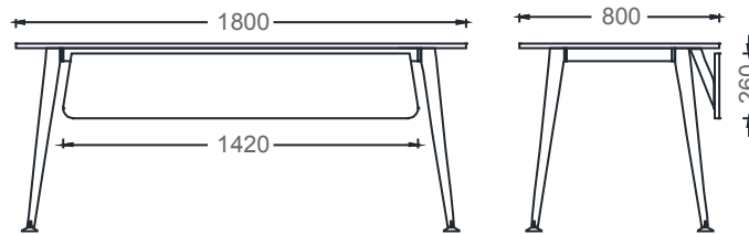
M4080180 - MIO SINGLE DESK 80x180
