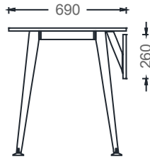
M3O70140 - MIO THREE-LEGGED SINGLE DESK 70x140
