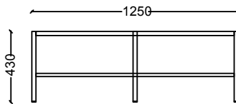
SSL60120 - SOLE RECTANGULAR COFFEE TABLE 120x60x43h
