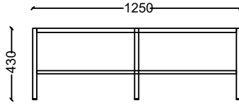
SSL60120 - SOLE DİKDÖRTGEN SEHPA 120x60x43h
