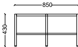
SSL8080 - SOLE KARE SEHPA 80x80x43h
