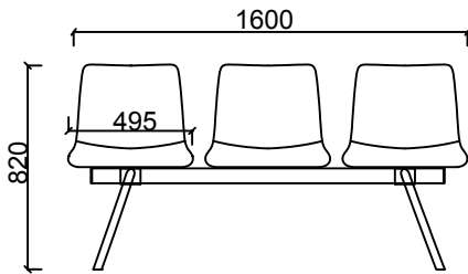
BRK2243 - BEST TRIPLE BENCH
