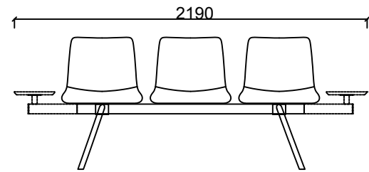
BRK2243S2 - BEST TRIPLE WITH TWO SIDE TABLES
