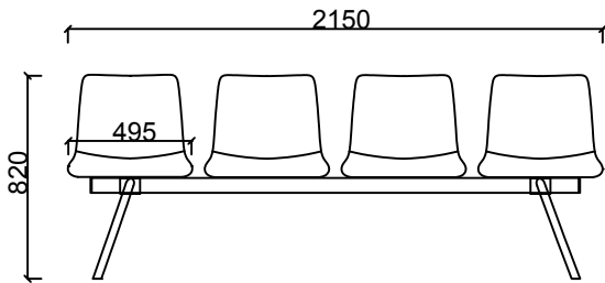
BRK2244 - BEST QUARTET BENCH
