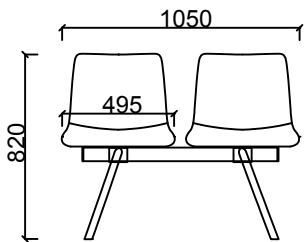
BRK2242 - BEST DOUBLE W/O SIDE TABLE
